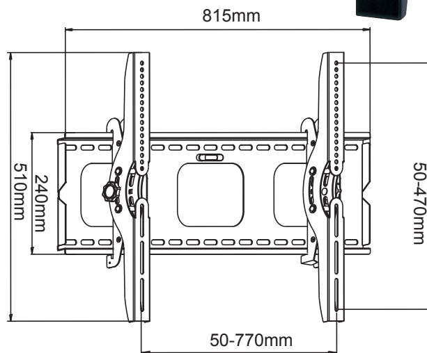
(Schematic Diagram)
